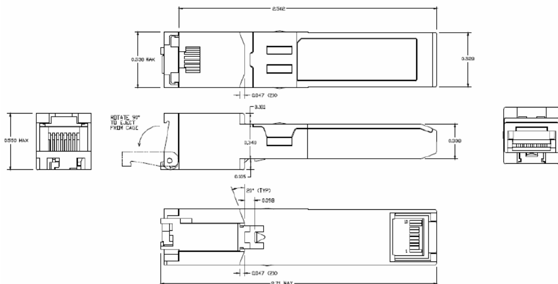
Figure2. GLC-T2 mechanical dimensions
